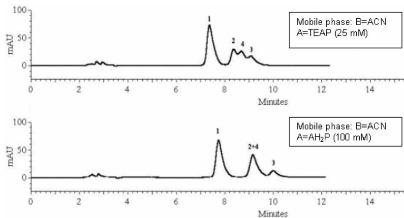
Figure 1. Effect of buffer type on separation of SGAs. Temperature: 26°C, Flow rate: 1.0 mL/min pH: 2.5 1: solasonine 2: \alpha -solanine 3: \alpha -chaconine 4: solamargine.
