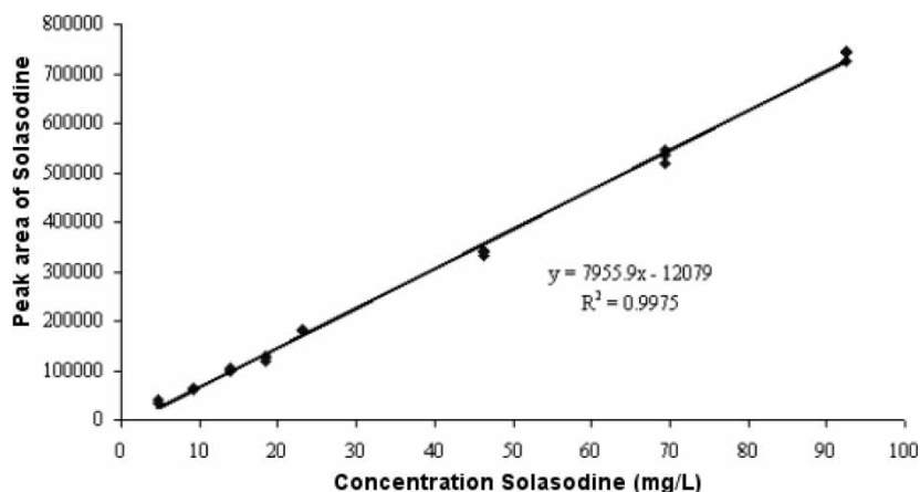
Figure 11. Calibration for solasodine in the concentration range of 4–100 mg/L without internal standard.
