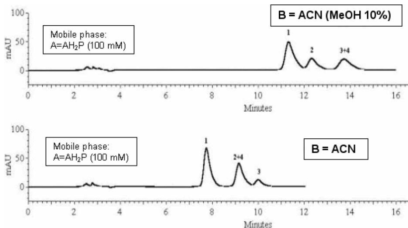
Figure 6. Methanol entrainer and separation of SGAs. Temperature 26°C, pH: 2.5 Flow rate: 1.0 mL/min 1: solasonine 2: \alpha -solanine 3: \alpha -chaconine 4: solamargine.
