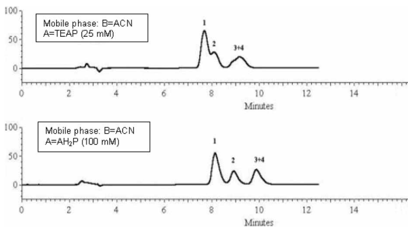
Figure 2. Effect of buffer type on separation of SGAs. Temperature: 50°C, pH: 2.5 Flow rate: 1.0 mL 1: solasonine 2: \alpha -solanine 3: \alpha -chaconine 4: solamargine.
