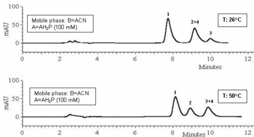
Figure 4. Effect of temperature (T) on the separation of SGAs. pH: 2.5, Flow rate: 1.0 mL/min 1: solasonine 2: \alpha -solanine 3: \alpha -chaconine 4: solamargine.
