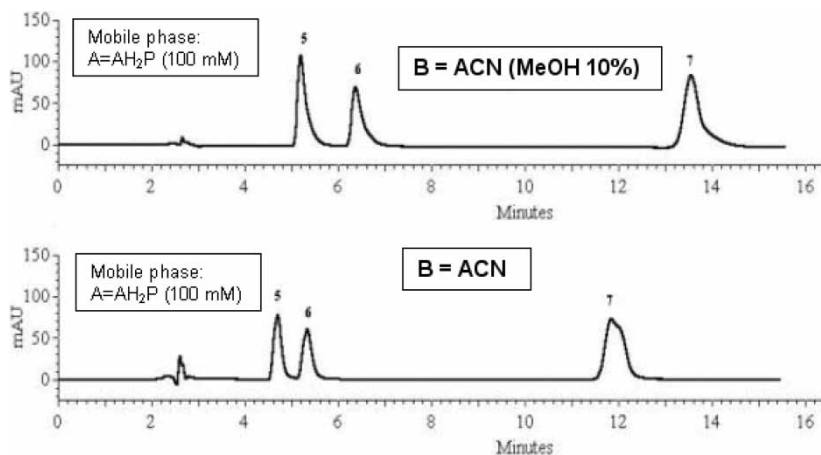
Figure 8. Methanol entrainer and separation of SGAs. Temperature: 50°C pH: 2.5 Flow rate: 1.0 mL/min 5: solanidine 6: solasodine 7: progesterone as internal standard.
