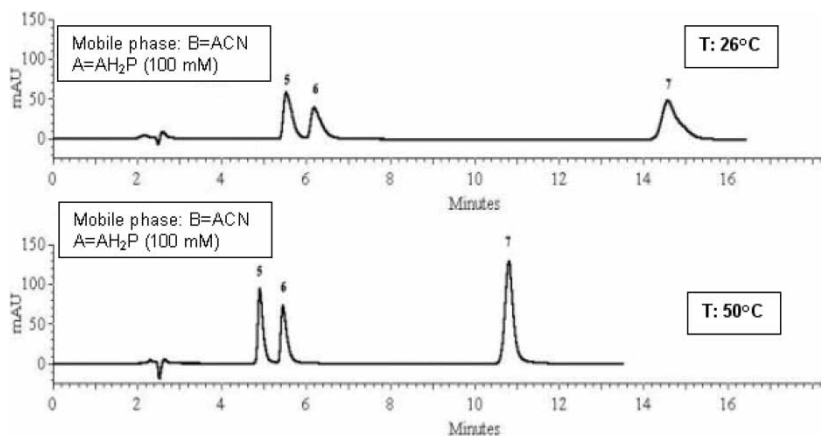
Figure 5. Effect of temperature (T) on the separation of SGAA. pH: 2.5 Flow rate: 1.0 mL/min 5: solanidine 6: solasonine 7: progesterone (internal standard).
