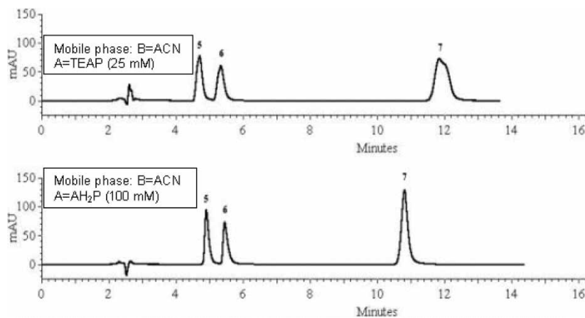
Figure 3. Effect of buffer type on the separation of SGAA. Temperature: 50°C, pH: 2.5 F: 1.0 mL/min 5: solanidine 6: solasodine 7: progesterone (internal standard).
