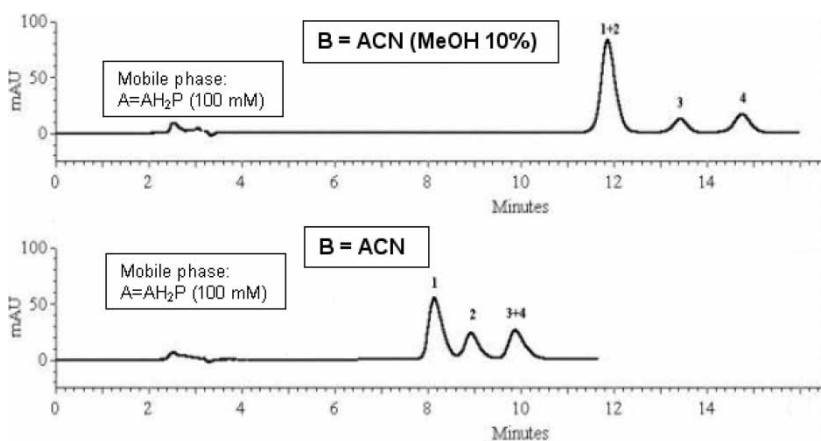
Figure 7. Methanol entrainer and separation of SGAs. Temperature 50°C, pH: 2.5 Flow rate: 1.0 mL/min 1: solasonine 2: \alpha -solanine 3: \alpha -chaconine 4: solamargine.
