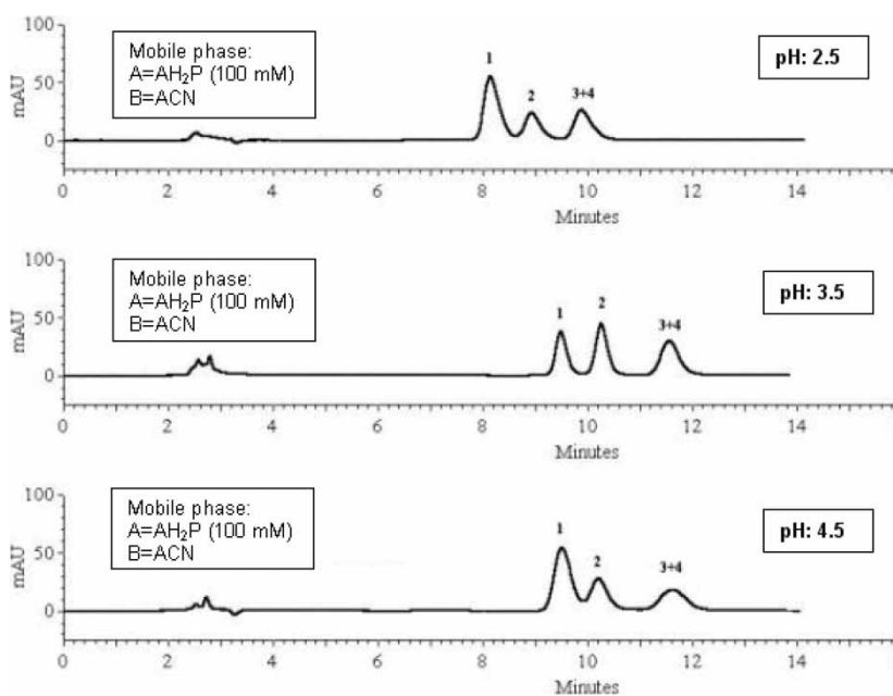
Figure 9. Effect of pH on the separation of SGAs. Temperature: 50°C Flow rate: 1.0 mL/min 1: solasonine 2: \alpha -solanine 3: \alpha -chaconine 4: solamargine.
